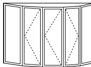
10° Bow - Fixed/Casement/Casement/Casement/Fixed
